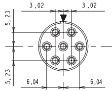
14-7 6 contacts + ground 7 x Ø1.6 (#16)
