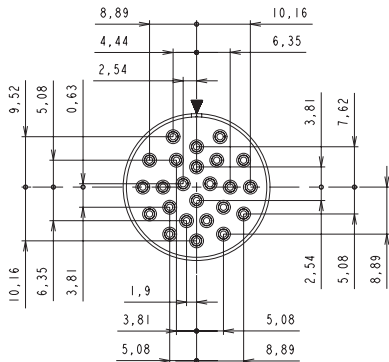
20-24 24 contacts 24xØ1.0 (#20)
