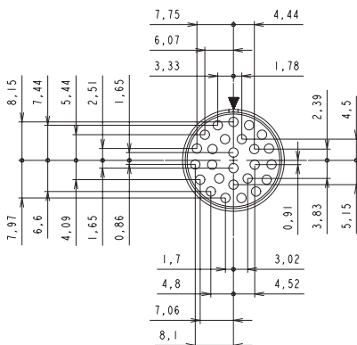
16-26 26 contacts 26 x Ø1.0 (#20)
