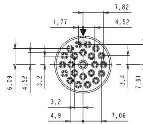
16-23 23 contacts 22 x Ø1.0 (#20) + 1 x Ø1.6 (#16)
