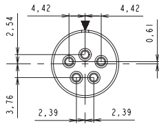
14-5 5 contacts 5 x Ø1.6 (#16)
