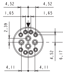
14-12 12 contacts 8 x Ø1.0 (#20) + 4 x Ø1.6 (#16)
