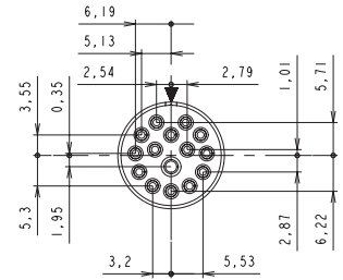
14-15 15 contacts 14 x Ø1.0 (#20) + 1 x Ø1.6 (#16)
