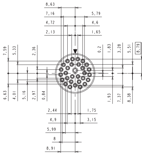
18-30 30 contacts 29xØ1.0 (#20) 1xØ1.6 (#16)
