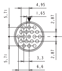
14-19 19 contacts 19 x Ø1.0 (#20)
