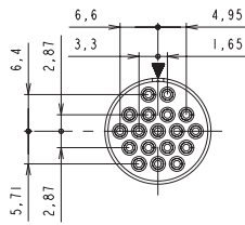
14-18 18 contacts 18 x Ø1.0 (#20)
