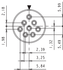
16-8 8 contacts 8 x Ø1.6 (#16)
