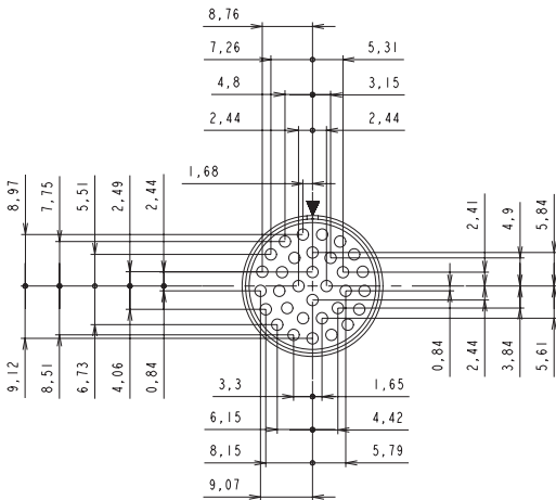
18-32 32 contacts 32xØ1.6 (#16)
